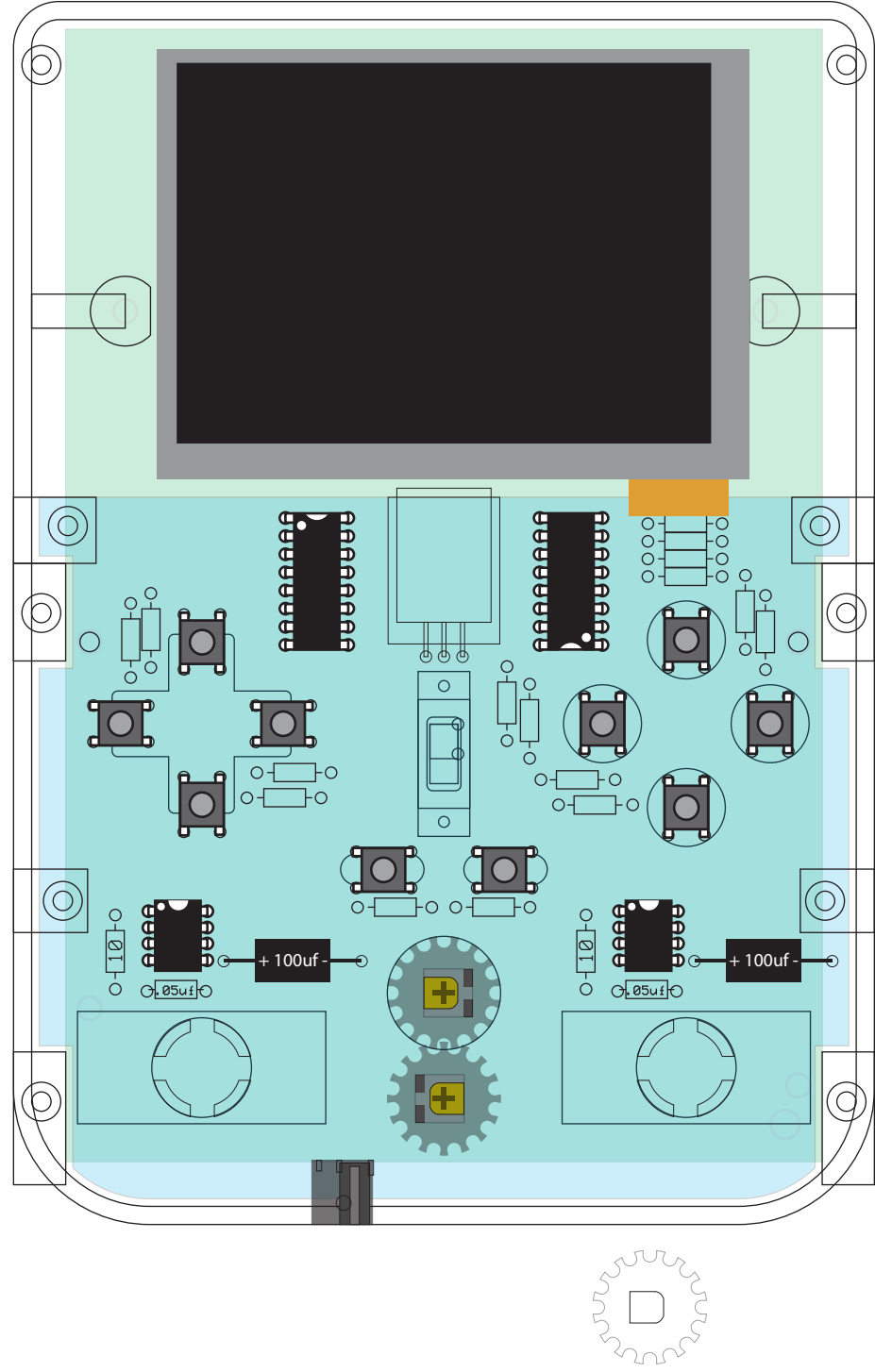
FRONT (as viewed from front) INTERNAL VIEW / MECH
