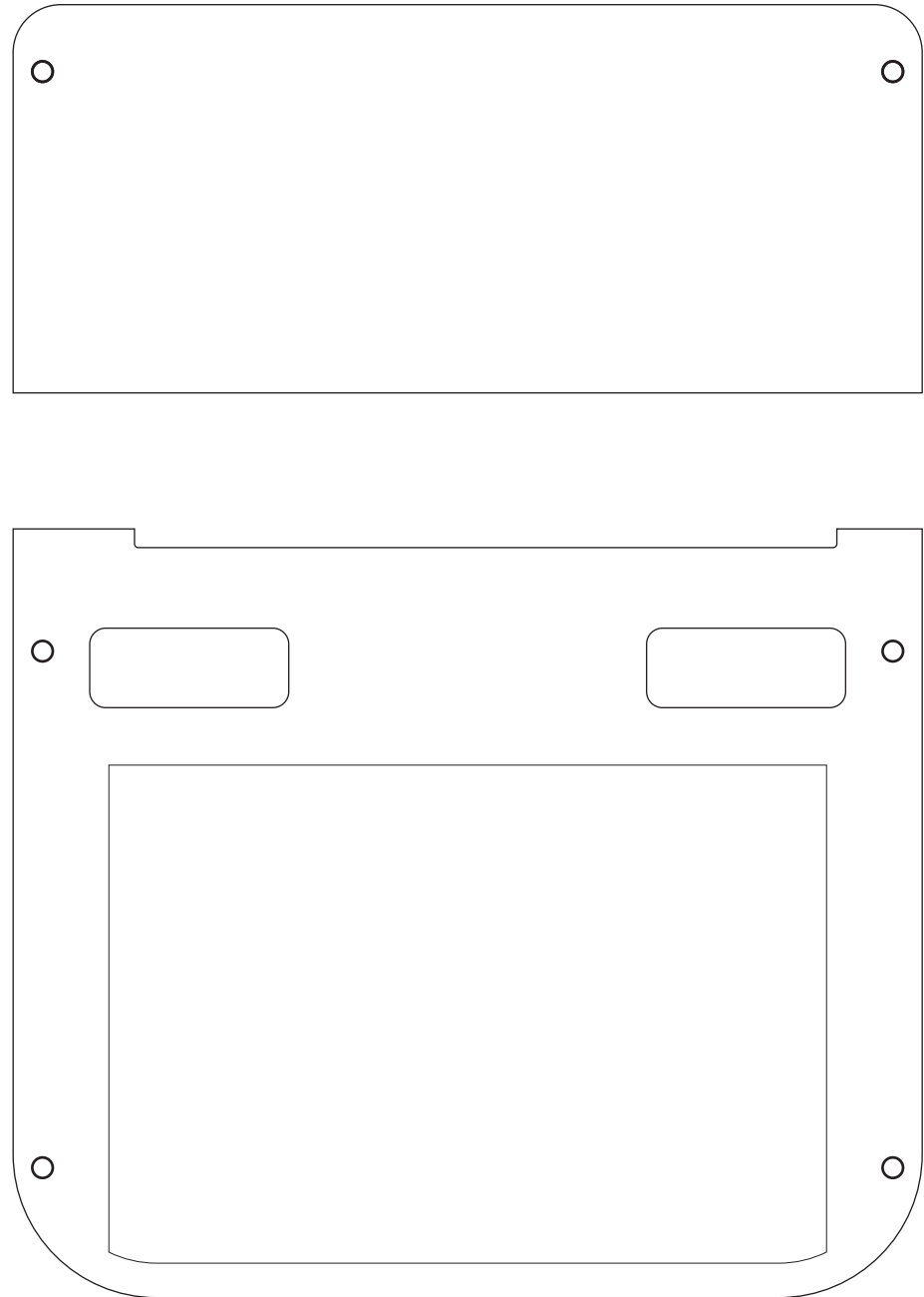
REAR PLATES (viewed from colored surface)
