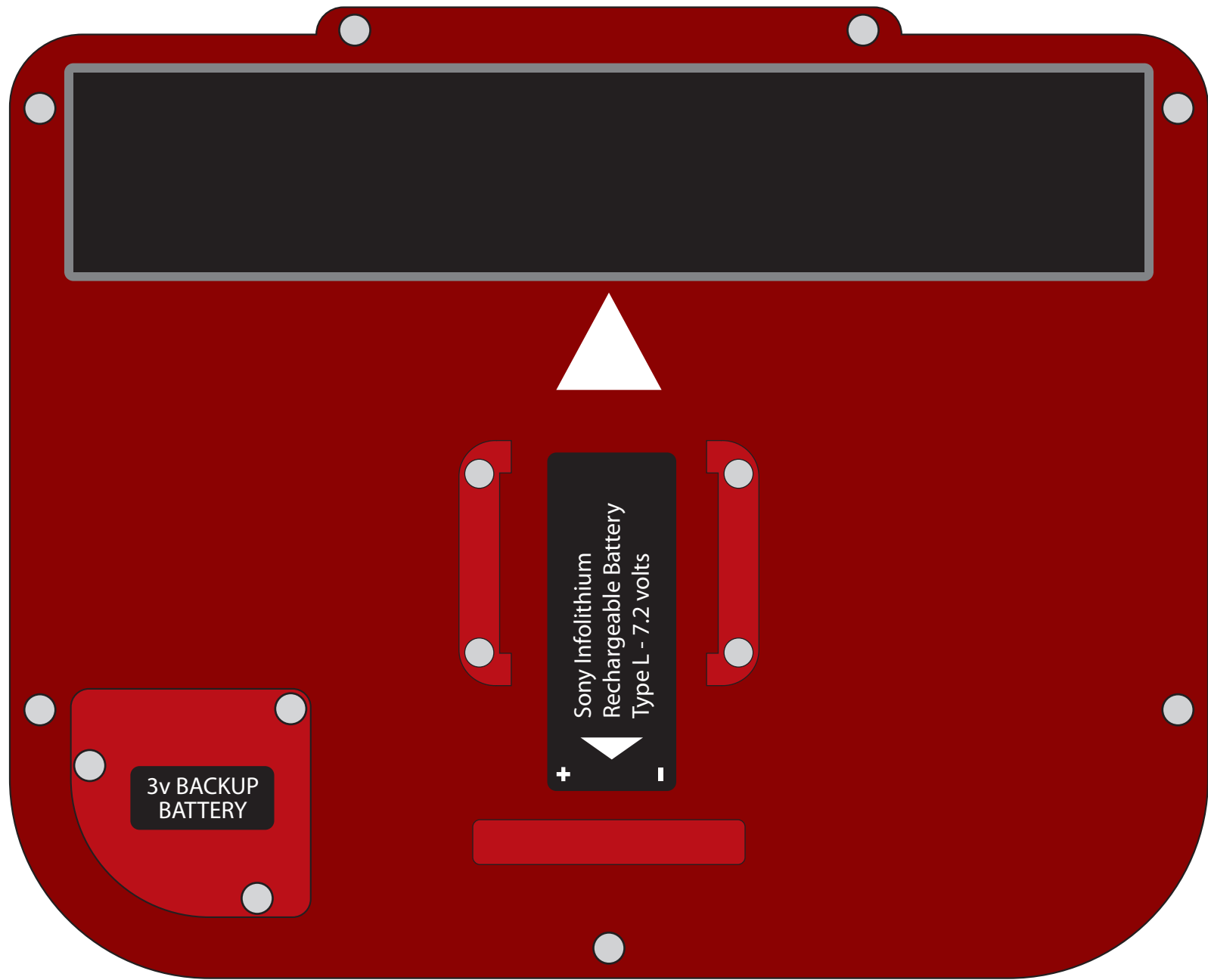
Rear Detail Layout, from rear
