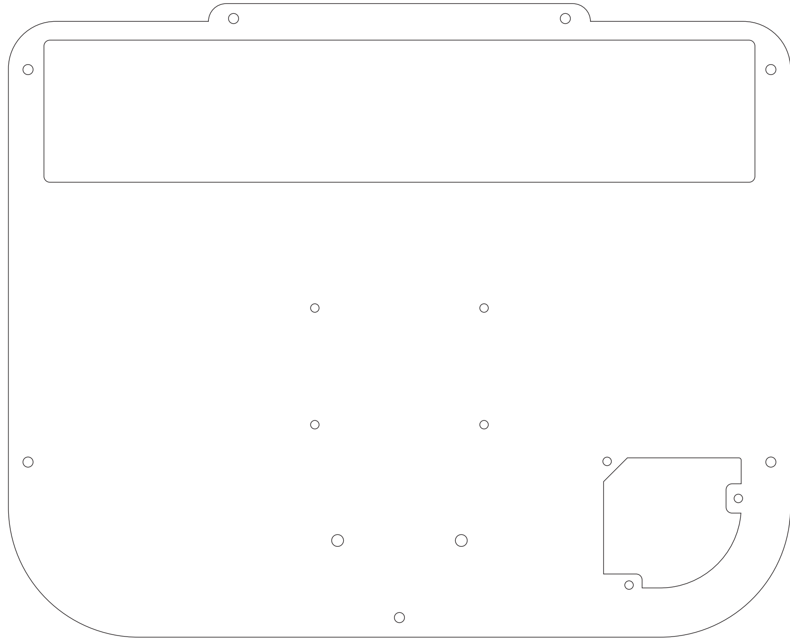
Rear plate. Rout from FRONT
