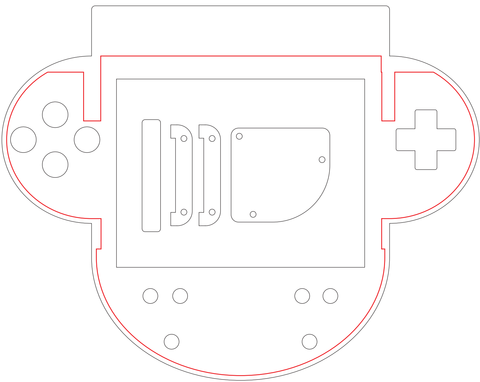
Front Red Plate Rout Reversed with Guide Notches
